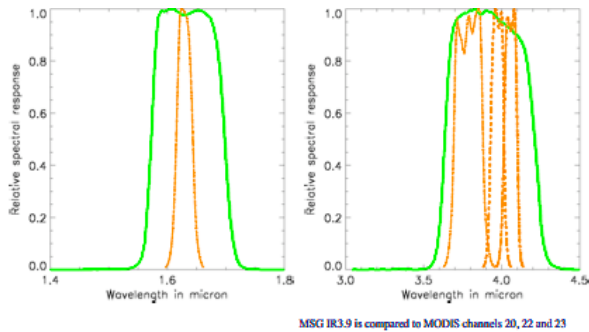
MSG IR3.9 is compared to MODIS channels 20, 22 and 23
