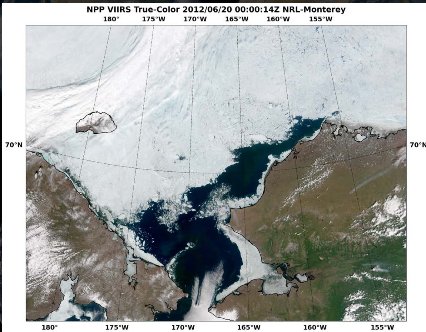
True color image example for the Arctic (Chukchi Sea) on 20 June 2012. (Image courtesy of Jeff Hawkins, NRL, Monterey)
