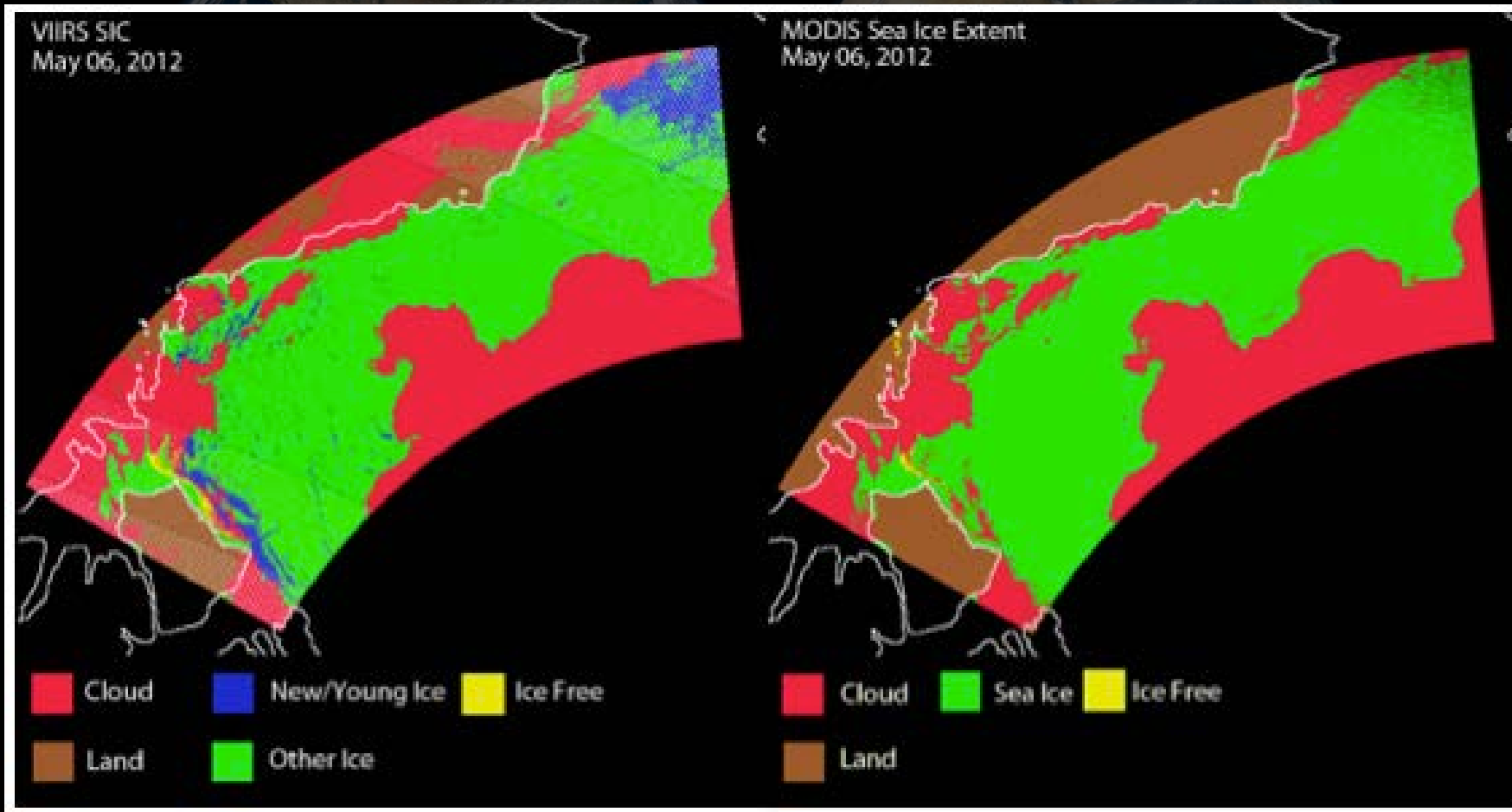
VIIRS Sea Ice Characterization EDR (left) and MODIS Sea Ice Extent (right) over the Beaufort Sea during May 6, 2012.
