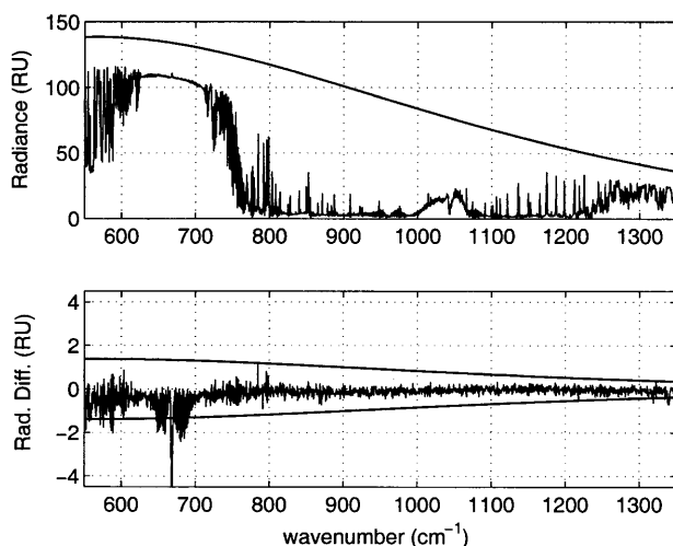
FIG. 7. Coincident clear-sky comparison between AERI-04 (Hillsboro) and the AERI prototype (AERI-00) at UW-SSEC on 7 Dec 1998 at Madison, WI. (top) The overlay of the AERI-04 observed downwelling radiance spectra and a Planck function at the AERI-04 ambient blackbody temperature. (bottom) The radiance difference between AERI-04 and AERI-00 averaged over the 1-h period 1624–1724 UTC. For reference, \pm 1\% of the AERI-04 ambient blackbody radiance is represented by the solid lines. [Radiance units: \text{RU} = \text{mW} (\text{m}^2 \text{sr cm}^{-1})^{-1} .] See the text for an explanation of the differences in the 660–680- \text{cm}^{-1} region.
