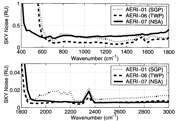
FIG. 13. Noise on three calibrated clear-sky scenes observed by the AERI. The curves show the real-time sky noise product from the AERI-01 system at the SGP CF on 18 Sep 2000, the AERI-06 instrument at the TWP-Nauru site on 15 Nov 1998, and the ER-AERI (-07) at the NSA-Barrow site on 10 Mar 1999. [Radiance units: RU = mW (m 2 sr cm -1 ) -1 .]
