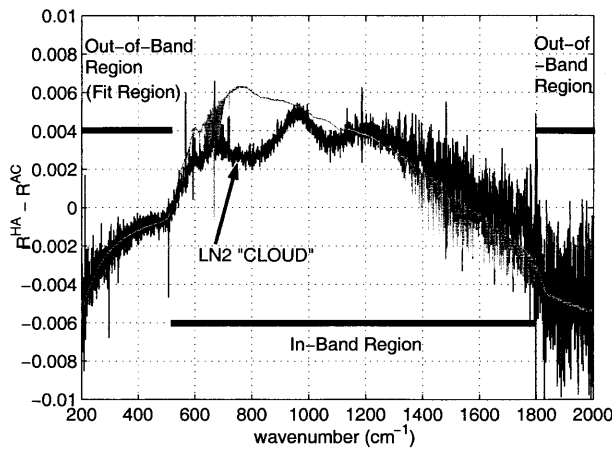
FIG. 1. The nonlinearity model fit (gray curve) to a measured responsivity difference between hot/ambient and ambient/LN2 reference targets. The fit region is 200–460 \text{cm}^{-1} , which avoids the “in-band” uncertainties of the LN2 target emissivity due to a liquid water cloud that forms over the cold target. Note that the quadratic nonlinearity model agrees in both the 200–460- and 1800–2000- \text{cm}^{-1} out-of-band regions even though the least squares fit only uses the first region to determine a_2 . The test data are of AERI-05 on 8 Dec 1998 but are typical of all standard AERI systems. Units are instrument counts per radiance unit [counts per \text{mW} (\text{m}^2 \text{sr cm}^{-1})^{-1} ].
