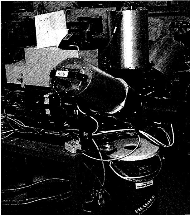
FIG. 5. Typical UW-SSEC laboratory end-to-end calibration verification using reference targets at about 318 (zenith view) and 273.15 K (nadir view). This “four body” test was used to verify the radiometric calibration of the AERI instruments prior to deployment of the systems to the DOE ARM sites.
