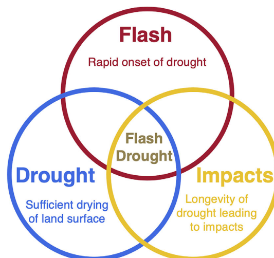
FIGURE 1 A Venn diagram illustrating the triad of components that form the basis of flash drought. The intersection of these three components (flash, drought, and impacts) defines a flash drought event.
