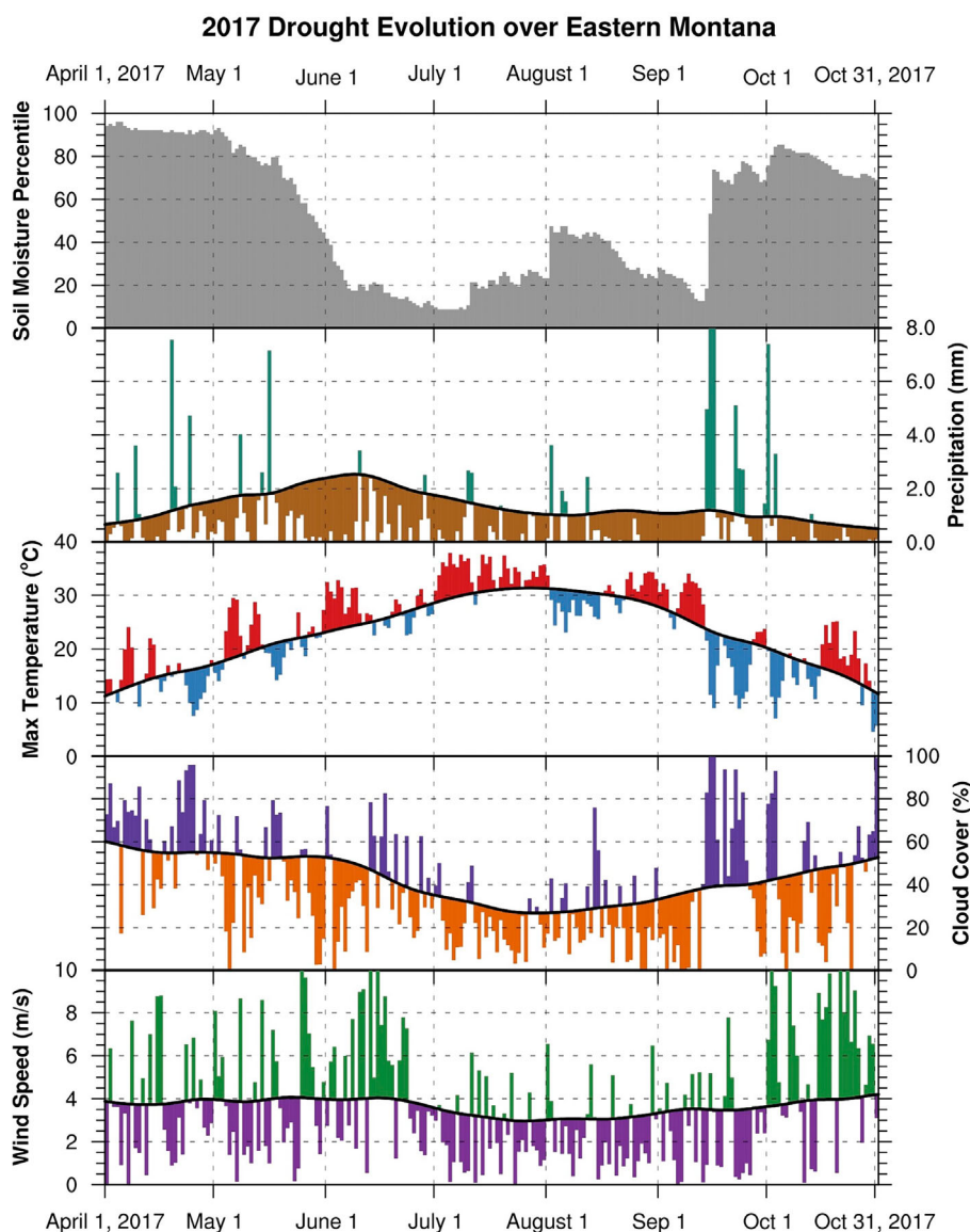
FIGURE 2 Times series of flash drought evolution in Eastern Montana in 2017. For Eastern Montana (defined as the region bounded by 46° N–49° N and 109° W–104° W), from top to bottom: daily soil moisture percentile (calculated relative to data for 1916–2017); departures from the climatological average (1950–2017; solid black line) of daily precipitation (mm); departures from the climatological average (1950–2017; solid black line) of daily maximum temperature (°C); departures from the climatological average (1979–2017; solid black line) of mean daily cloud cover (%); and departures from the climatological average (1979–2017; solid black line) of mean daily horizontal 10-m wind speed (m/s) from April 1, 2017 to October 31, 2017 (from Hoell, Perlwitz, & Eischeid, 2019).
