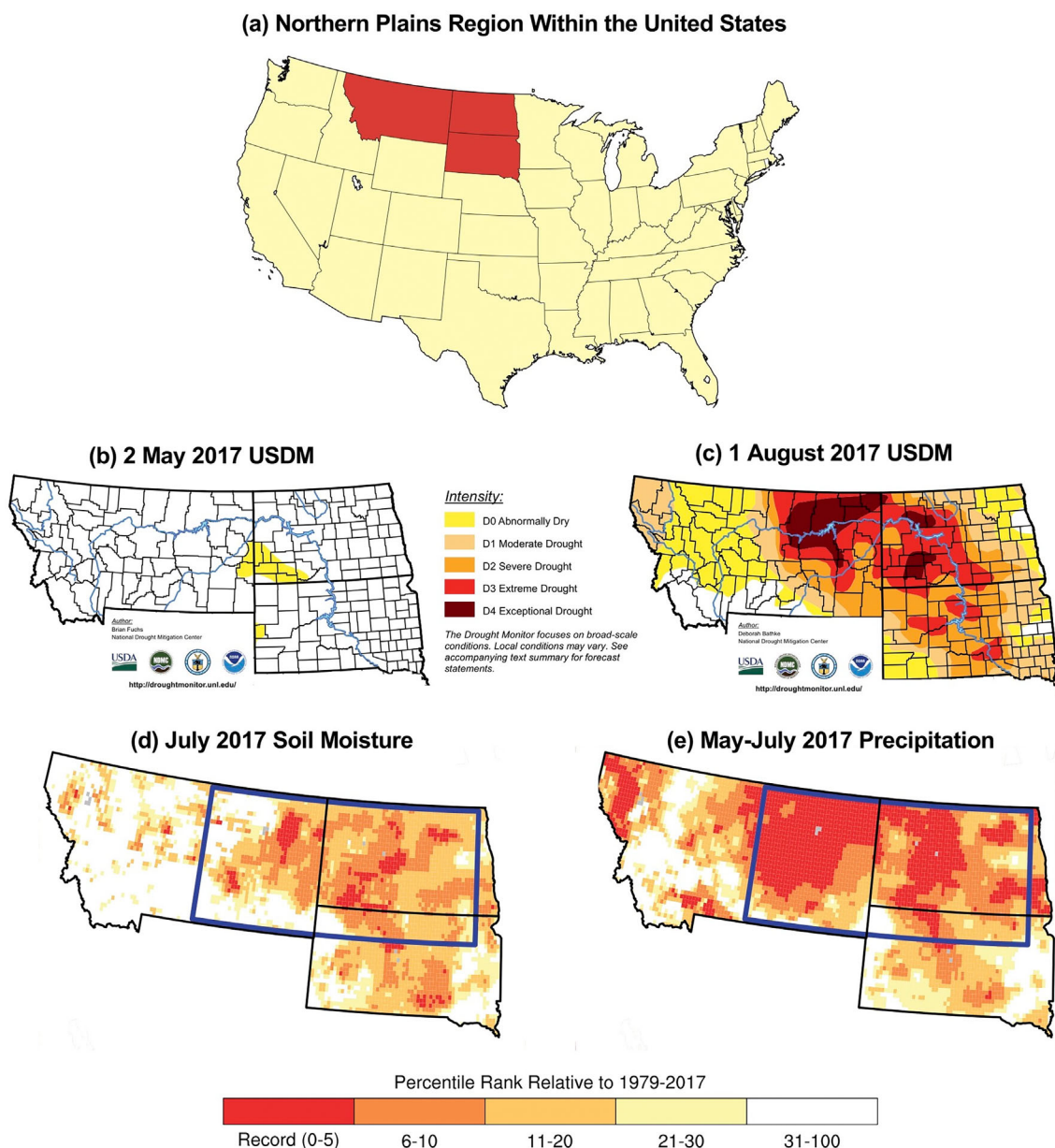
FIGURE 3 Spatial evolution of flash drought in the Northern Great Plains in 2017. (a) Location of the northern Plains as examined in the 2017 drought case study. (b, c) U.S. Drought Monitor on May 2 and August 1, 2017, respectively. Also shown are percentile ranks of (d) July 2017 1-m soil moisture and (e) May–July 2017 precipitation based on the NLDAS-2 data (from Hoell, Perlwitz, Dewes, et al., 2019). The blue boxes indicate the Northern Great Plains region studied in Hoell, Perlwitz, Dewes, et al. (2019).
