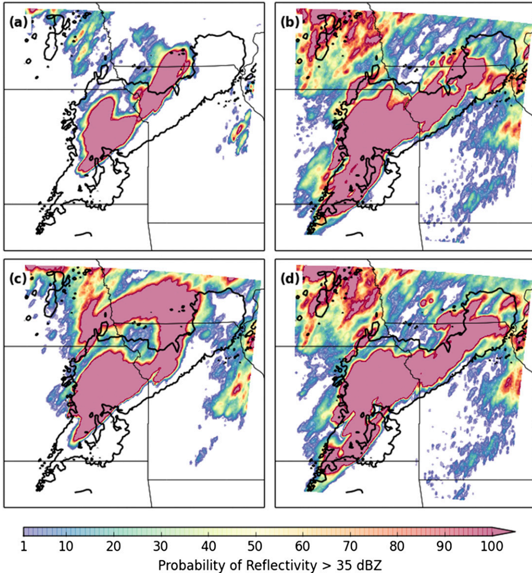
FIG. 10. Probability of composite radar reflectivity >35 dBZ during the 1-h forecast period for the (a) CTRL, (b) SAT, (c) RAD, and (d) SATRAD experiments. The composite reflectivity >35 dBZ swath from the TRUTH simulation is indicated by the thick black contour overlaid on each panel.
