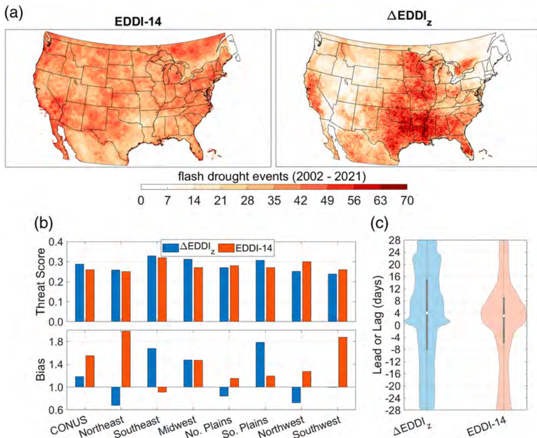
FIG. 6. (a) Maps of the climatological frequency of flash drought events between 2002 and 2021 identified by (left) EDDI-14 and (right) \Delta\text{EDDI}_z definitions. (b) Bar plots of the CONUS- and region-average TS and bias ratio of flash drought identification of (blue) \Delta\text{EDDI}_z and (red) EDDI-14. (c) Violin plots of the timing of hits of (blue) \Delta\text{EDDI}_z and (red) EDDI-14 flash droughts in comparison with the other nine indicators.
