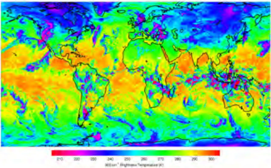
Figure 1. Data is flowing in from the Cross-track Infrared Sounder (CrIS) instrument aboard NASA's newest Earth-observing satellite, the Suomi National Polar-orbiting Partnership (NPP). This image is a composite of 900 cm -1 brightness temperatures from three days of CrIS data from January 21, 23 and 25, 2012. The orange colors represent very warm sea surface temperatures, while magenta represents both very cold temperatures as well as high-altitude cloud tops.
