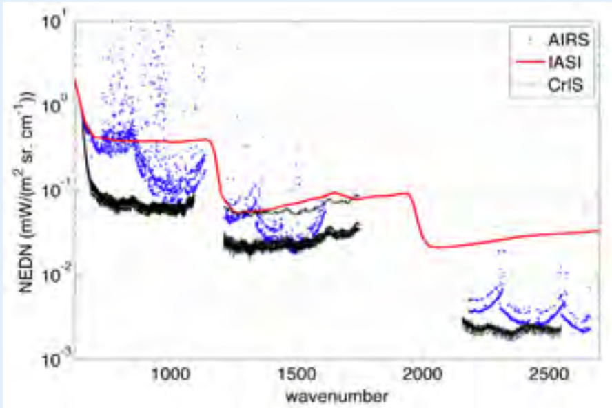
Figure 3. CrIS radiometric noise performance compared to AIRS and IASI.
