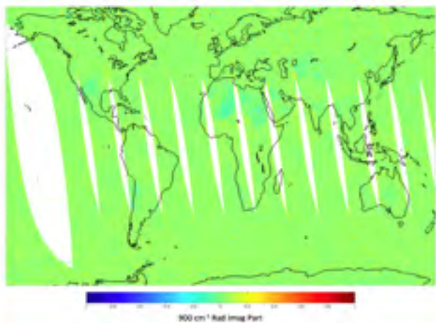
Figure 2. Imaginary parts of calibrated radiance spectra on 18 April 2012. The lack of structure and non-zero imaginary parts confirms the proper fringe counting of the CrIS interferometer and resulting radiometric calibration.
