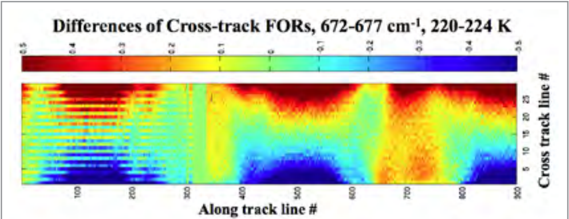
Figure 7. Longwave spectral region sweep direction biases on 18 April, with the at-launch numerical filter (prior to along track line # 300) and after upload of the new numerical filter.
