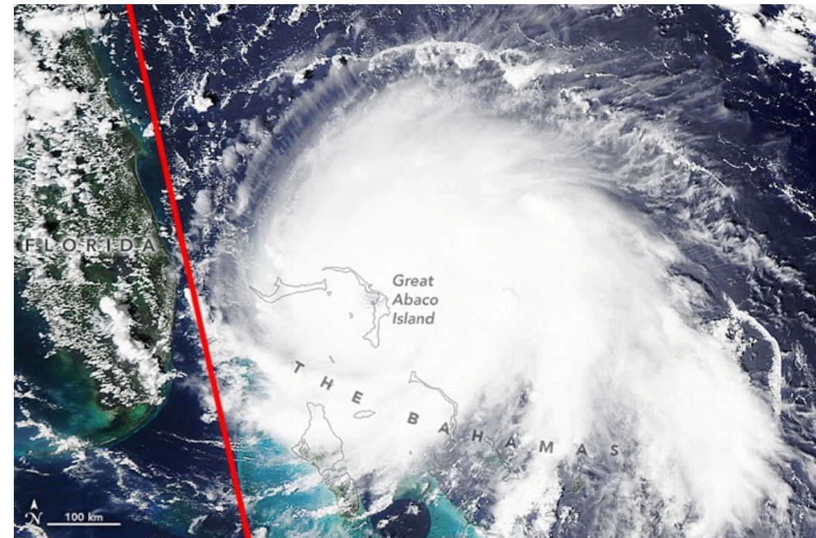
Aeolus satellite track overlaid on a NASA Aqua's satellite image of hurricane Dorian at 1805 UTC on September 1, 2019. (Image credit: NASA)
