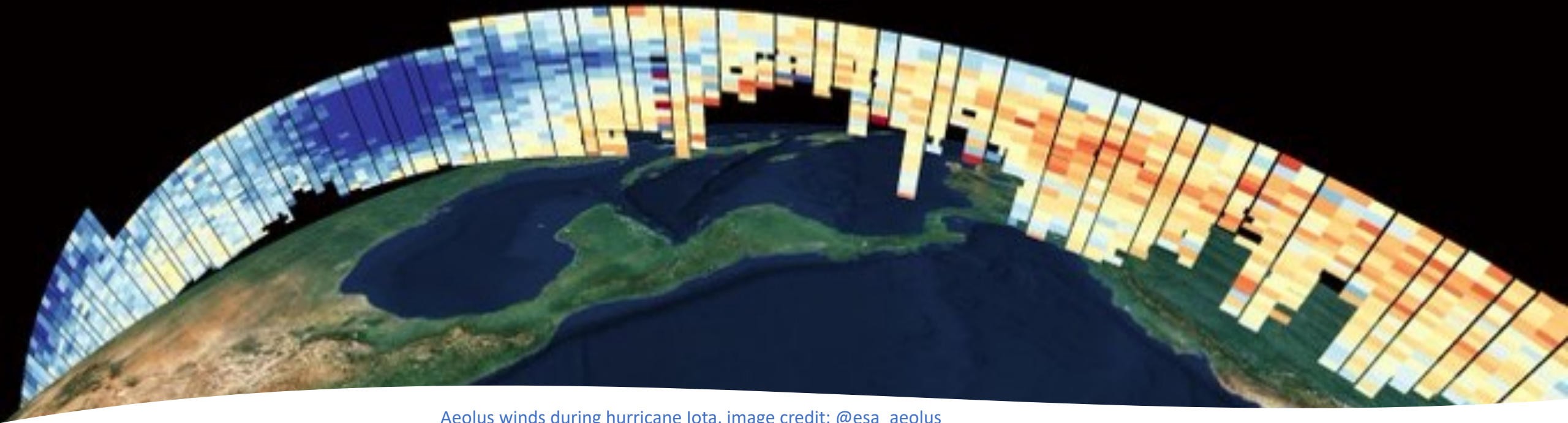
Aeolus winds during hurricane Iota, image credit: @esa_aeolus
