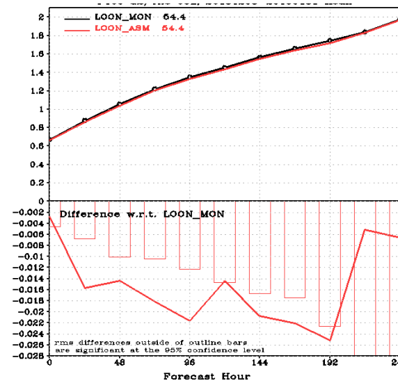
Tropical Temperature RMSE p=100 hPa
