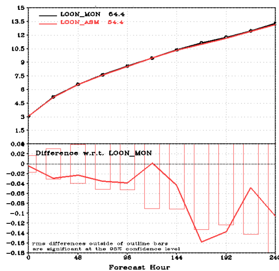
Tropical Wind RMSE p=200 hPa
