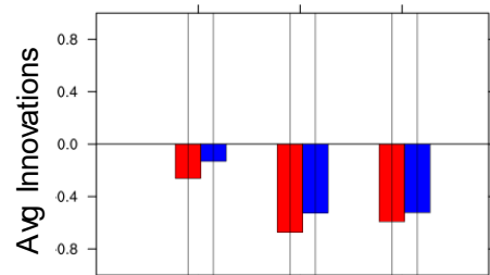
O-B Differences for U-wind (m/s) Tropics, p < 100 hPa
