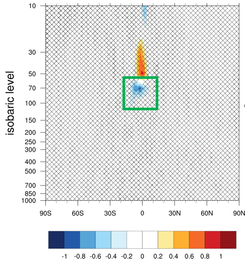
Zonal Wind (m/s) 24-hr Forecast
