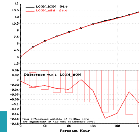
Tropical Wind RMSE 250 hPa
