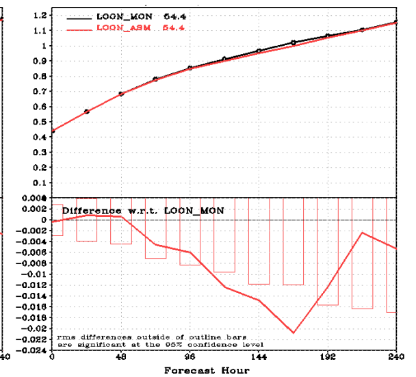
Tropical Temperature RMSE p=200 hPa
