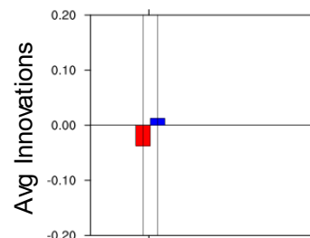
O-B Differences for Temperature (K) Tropics, p < 100 hPa
