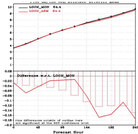
Tropical Wind RMSE p=100 hPa
