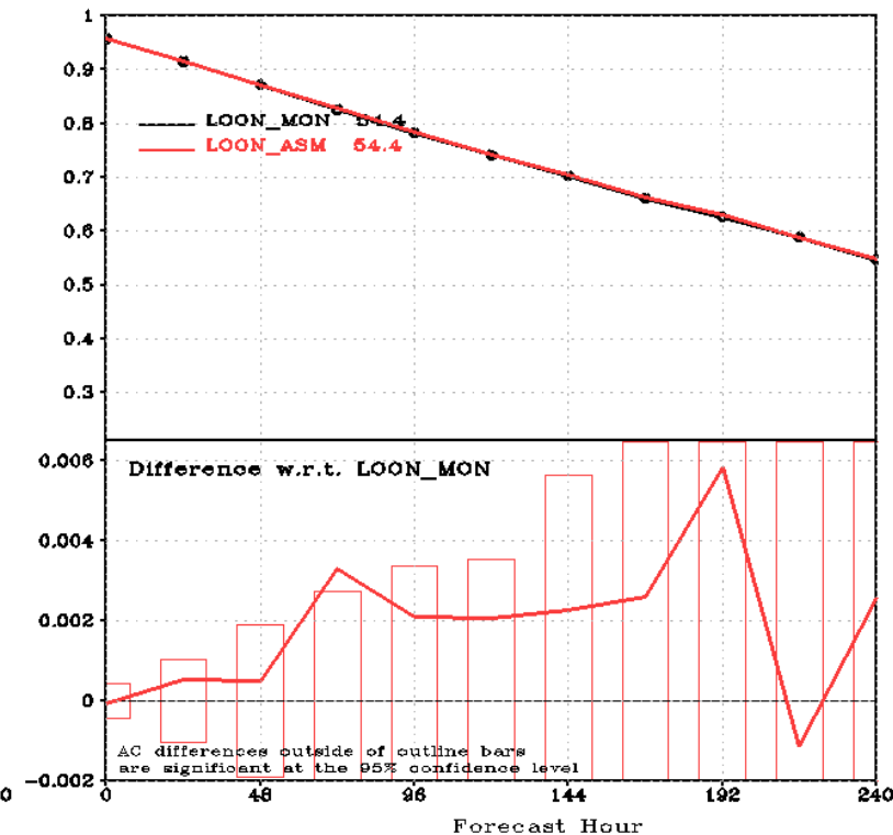
Tropical Temperature AC p=250 hPa
