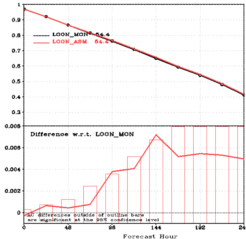
Tropical Wind AC p=250 hPa
