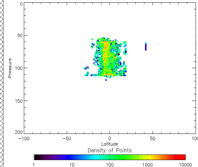
Number density of Loon winds
