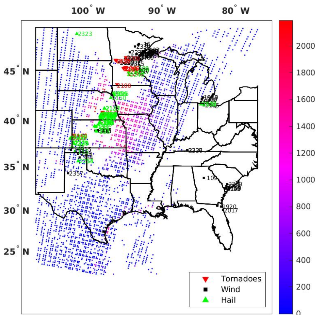
SPC Storm Report 12 Hours from IASI MUCAPE Data for 16z on 14-Aug-2020
