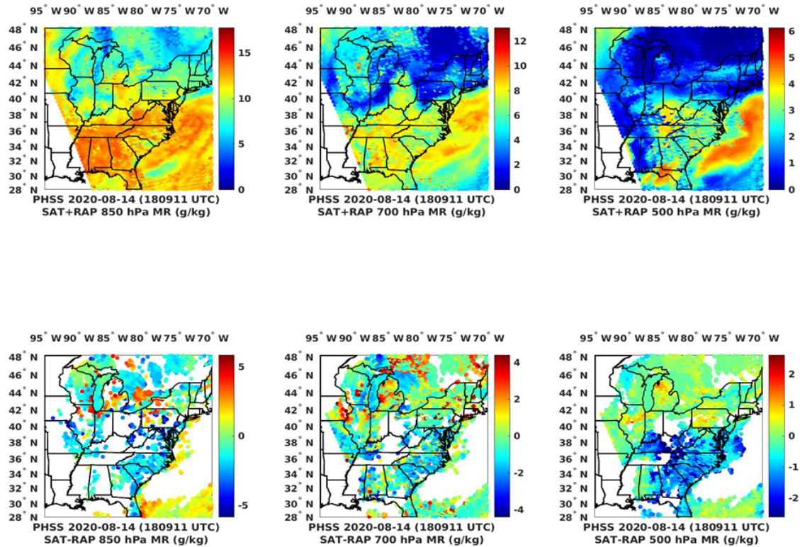
Figure 2. Polar satellite mixing ratio retrieval data produced at HU for August 14, 2020 at 18:09 UTC
