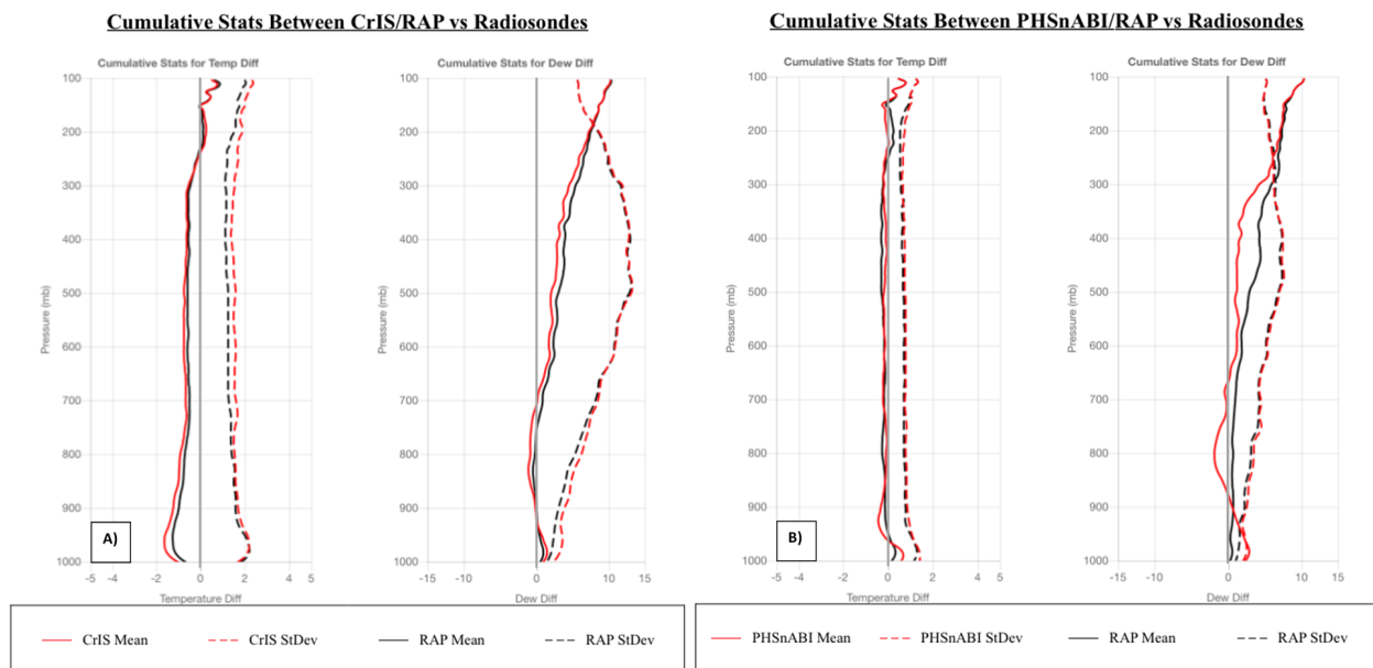
Figure 8A and B. July 2020 statistics showing mean and standard deviation temperature and dewpoint temperature differences between CrIS/RAP and radiosondes (left) and PHSnABI/RAP and radiosondes (right).
