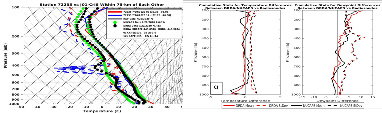
Figure 7C. The same as figure 7A and B, except these comparisons use data from J01-CrIS at 7:07 UTC and NUCAPS at 7:06 UTC.
