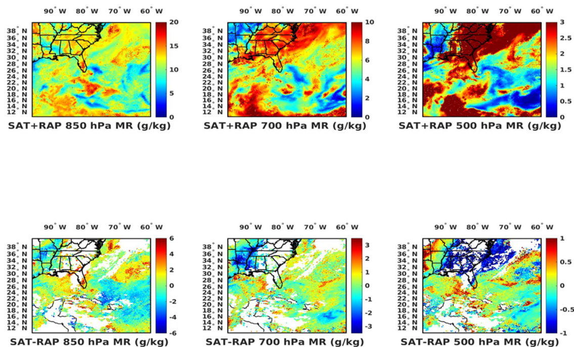
Figure 4. Mixing ratio data from PHSnABI produced for the TSHFD for August 15, 2020 at 2:44 UTC.
