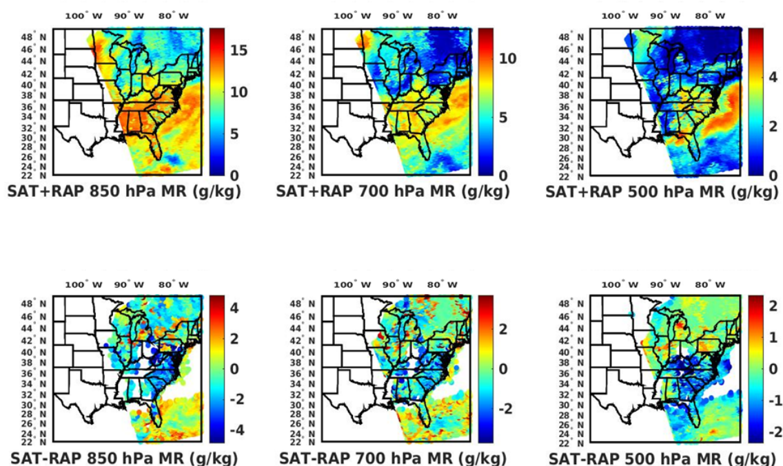
Figure 3. Polar satellite mixing ratio retrieval data produced at UW for August 14, 2020 at 18:09 UTC
