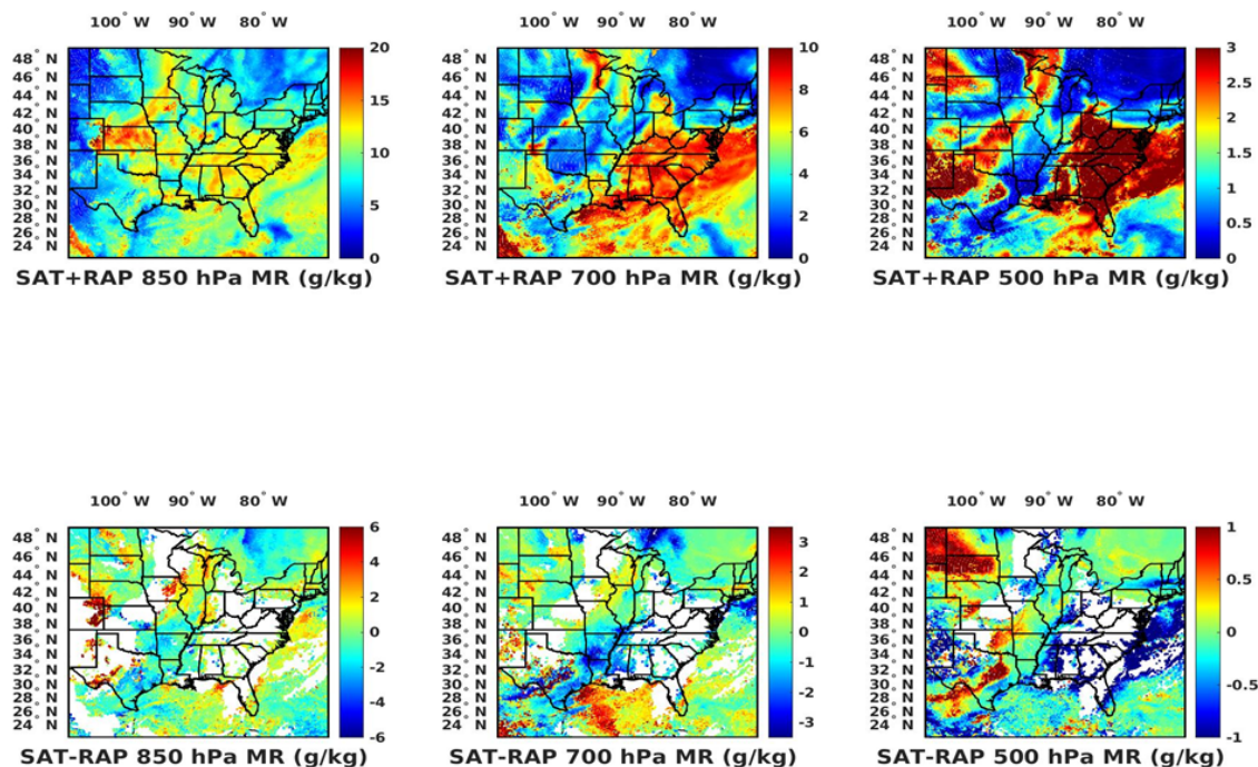
Figure 5. Mixing ratio data from PHSnABI produced at UW from August 15, 2020 at 2:44 UTC.
