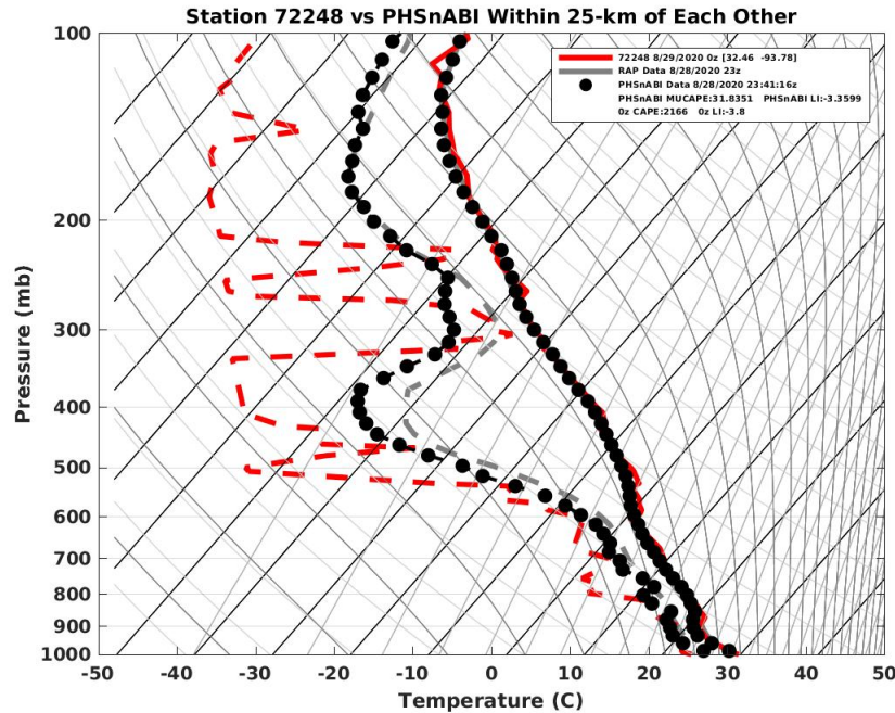
Figure 6b. Comparison between the 2-hr RAP forecast profile and PHSnABI satellite sounding with the radiosonde (station 72248) observation closest to the location chosen in figure 6a.
