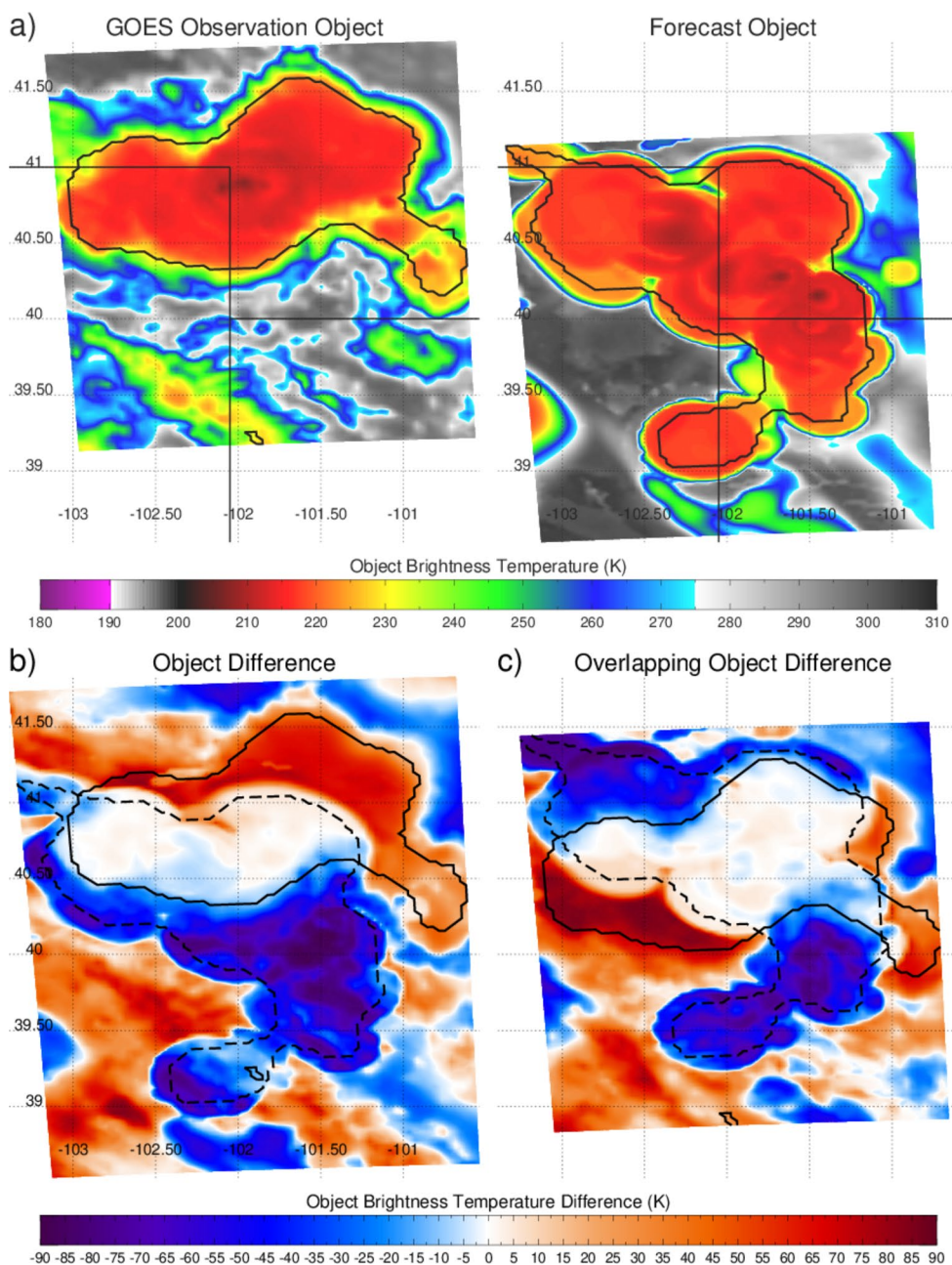
Figure 3. Example of removing displacement using the center latitude and longitude of Method for Object-Based Diagnostic Evaluation images. (a) Two matching object that are displaced. Difference between brightness temperatures when the objects (b) are not and (c) are overlapped. From Griffin et al. (2020). GOES, Geostationary Observing Environmental Satellite.
