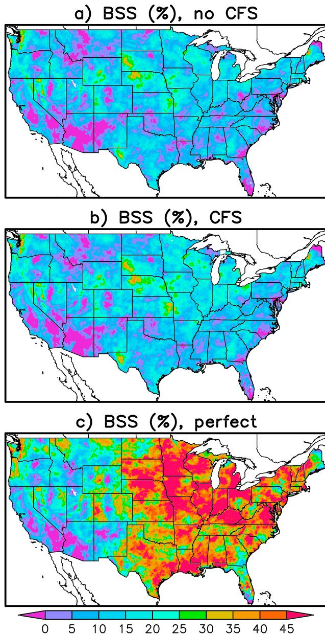
Figure 1. (a) Brier Skill Score (BSS) for the baseline four-week USDMM intensification forecasts using current and past data only (no CFS forecasts). (b) As in (a) but with CFS forecasts fields added as predictors. (c) As in (b) but with future observations substituted for CFS forecasts. This panel shows potential predictability possible from a perfect CFS forecast.
